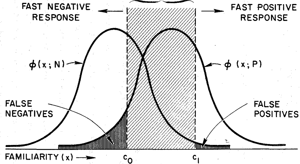
Figure 4. Distributions of familiarity values for distractor items, \phi(x;N) , and target items, \phi(x;P) .
