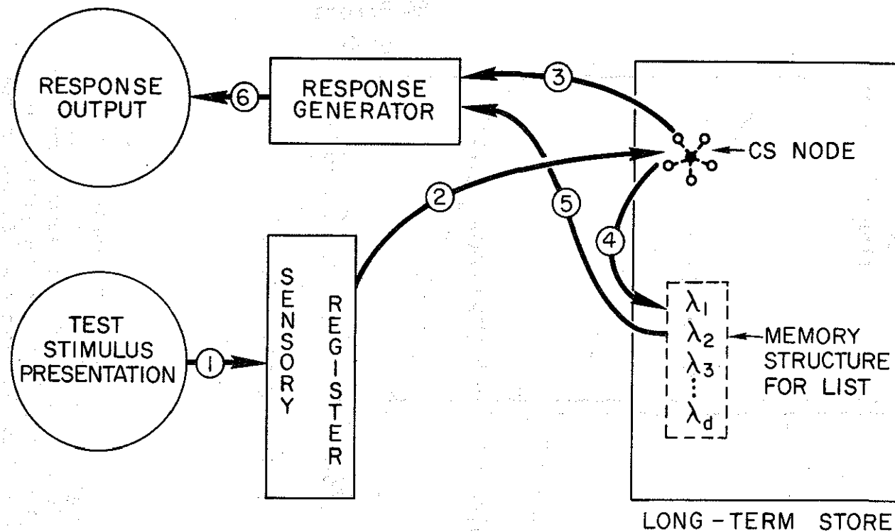
Figure 10. A schematic representation of the search and decision processes in long term recognition memory. A test stimulus is presented (1) and then encoded and matched to an appropriate CS node (2). The familiarity index associated with the node may lead to an immediate decision (3) and in turn to a response (6). Otherwise, an extended search of the stored target list is initiated (4), which eventually leads to a decision (5) and a subsequent response (6). Path (1), (2), (3), (6) represents a much faster response process than path (1), (2), (4), (5), (6), and one that is independent of target set size.
